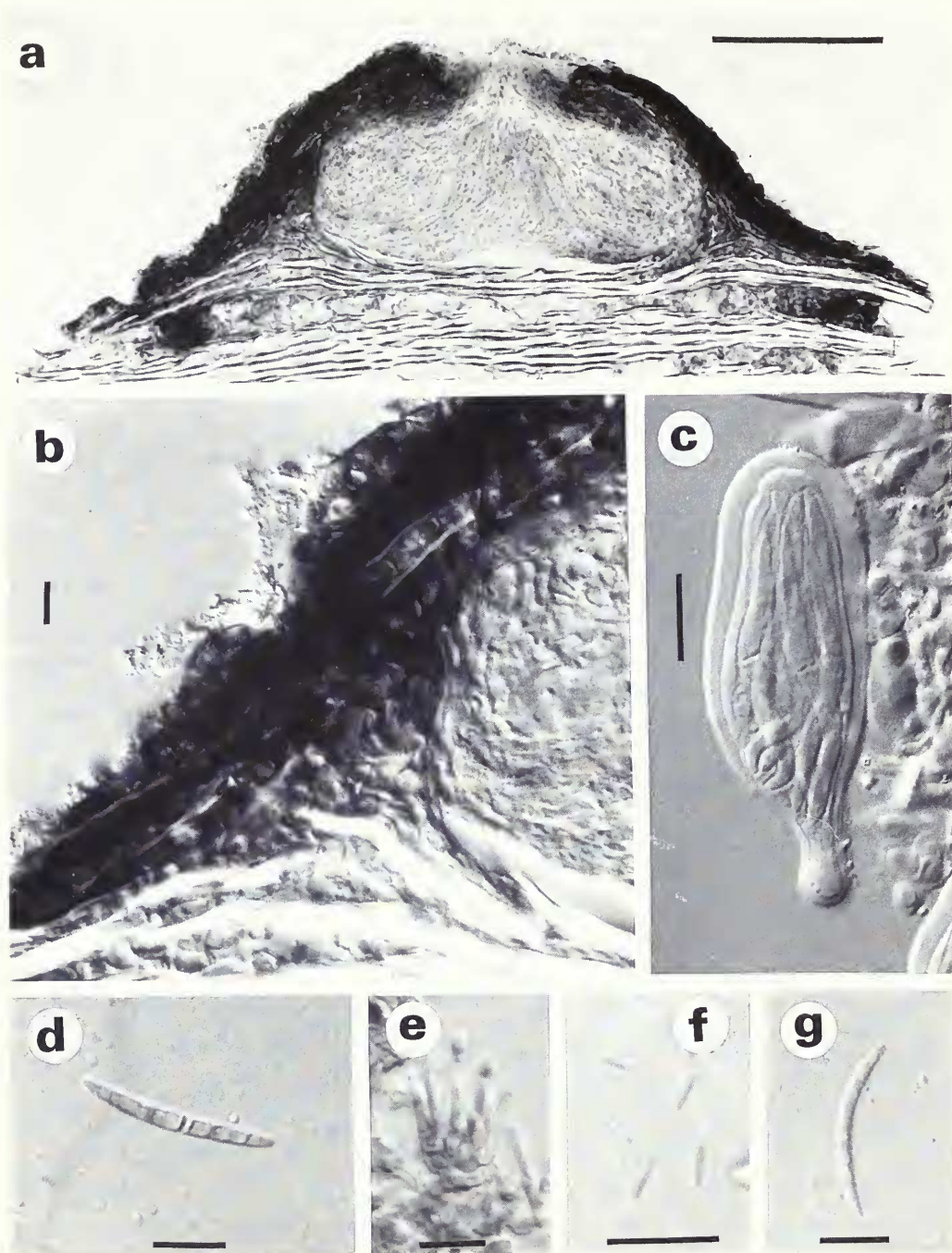
Fig. 8 Leptorhaphis epidermidis (Ach.) Th. Fr. (H-NYL 7503—holotype of Verrucaria oxyspora ) (a) Vertical section of ascoma showing basal fringe; scale = 100 µm; (b) Involucellum consisting of clypeate tissue; (c) Ascus and ascospores; (d) Ascospore; (e) Conidiogenous cells and microconidia; (f) Microconidia; (g) Macroconidia; scale = 10 µm.
